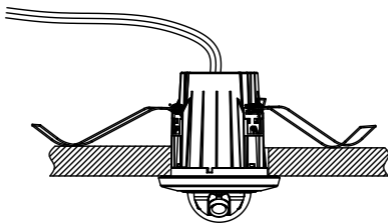
Figure 2-6 Complete the Installation
