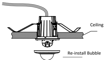
Figure 2-5 Re-install the Bubble
