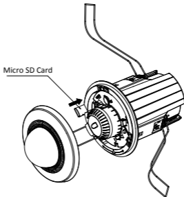
Figure 1-4 Install the SD Card
